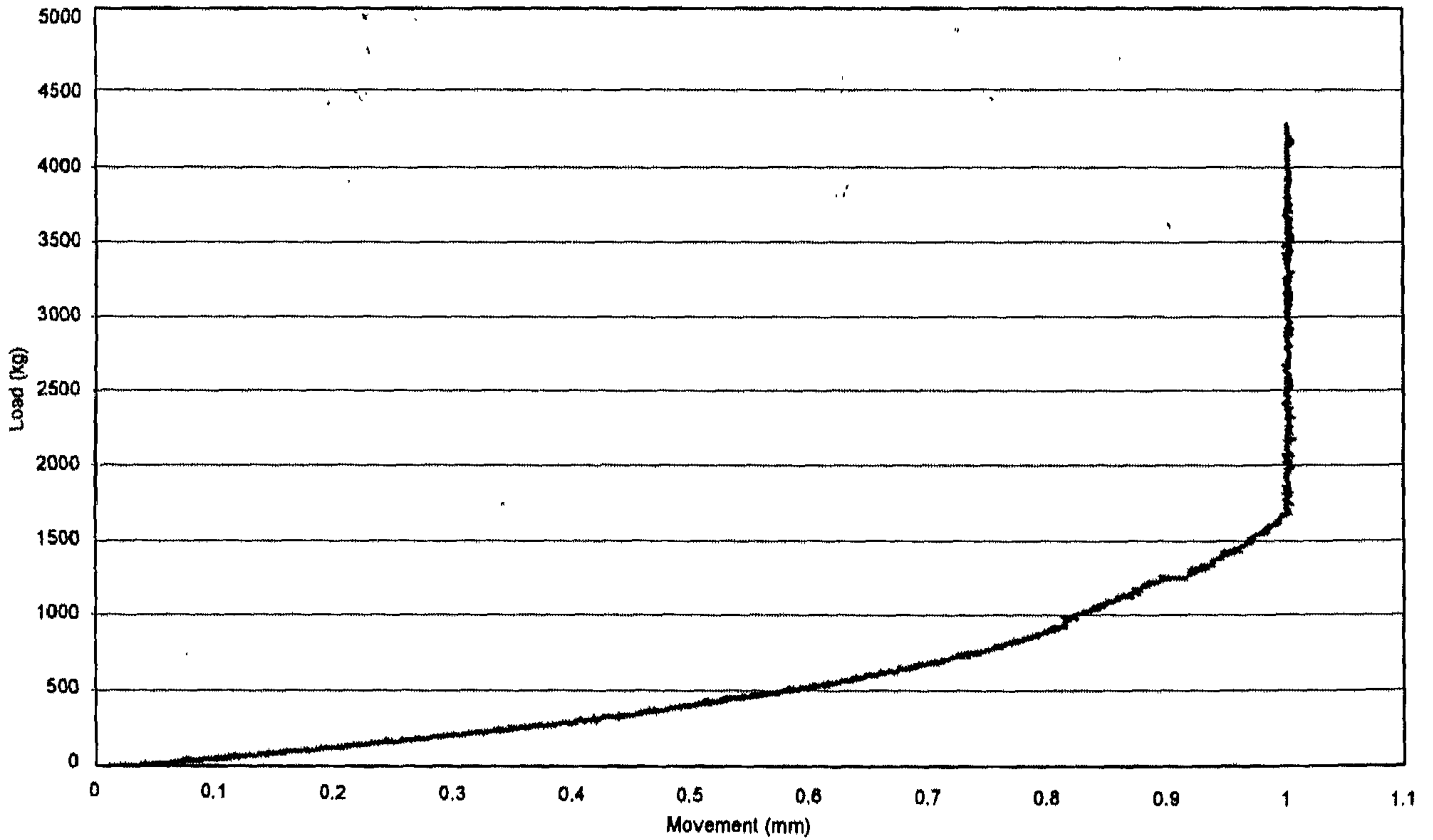
Load-Movement Curve (Sample No. awm)
